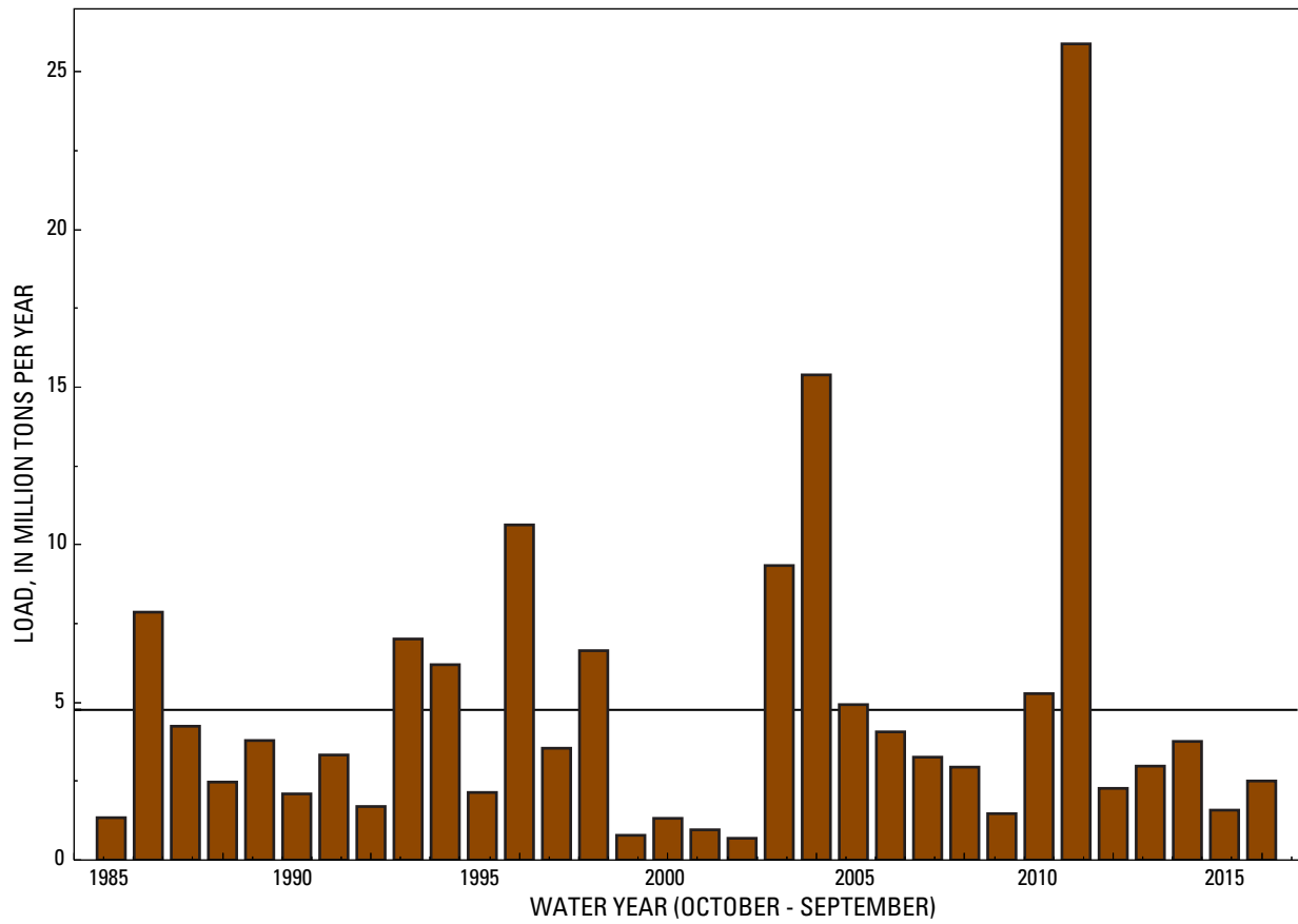
Figure 5. Combined annual suspended-sediment load delivered from the nine River Input Monitoring stations to the Chesapeake Bay. Black line represents the mean annual combined load of 4.76 million tons per year.
