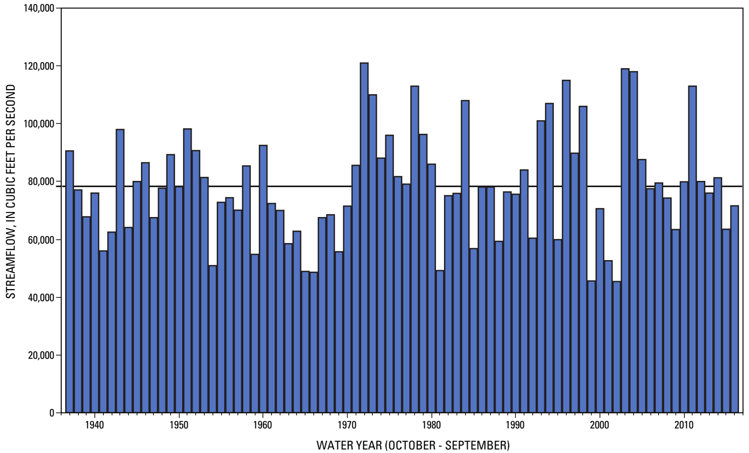
Figure 2. Estimated annual-mean streamflow entering Chesapeake Bay. Black line represents the average annual-mean streamflow of 78,476 cubic feet per second. Source http://md.water.usgs.gov/waterdata/chesinflow/wy/
